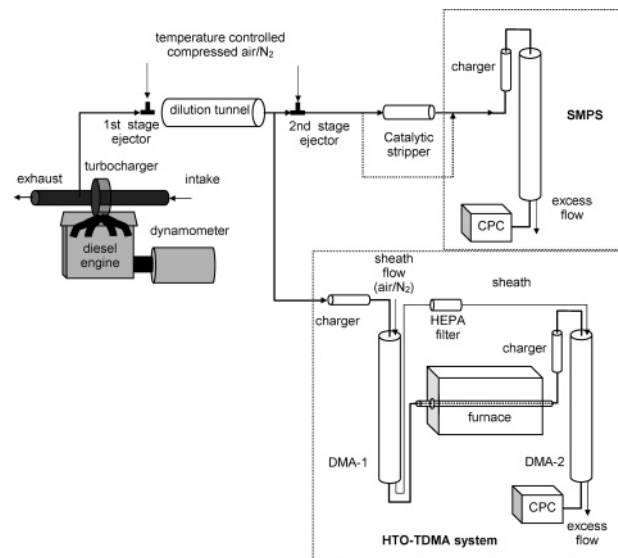
FIGURE 1. Schematic diagram of experimental setup. The bold line indicates the path taken by the diesel particles.
