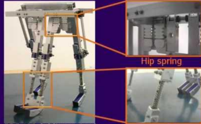
Leg spring
