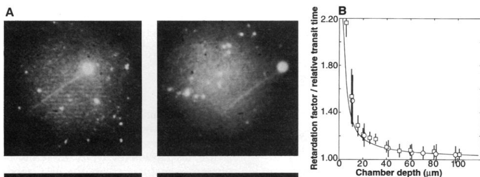
Fig. 2. (A) Magnetic beads tethered by single DNA molecules stained with ethidium as seen in a fluorescence microscope equipped with an image-intensified video camera (3). The beads were forced upward by flow and pulled to the right by a magnet. The mean diameter of the streptavidin-coated polystyrene paramagnetic beads (Dynabeads
