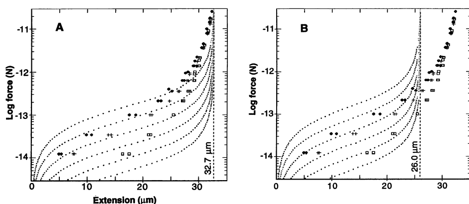
Fig. 4. (A) Semilogarithmic plot of force versus extension for a single \lambda -dimer molecule in three different \text{Na}^+ concentrations (from \text{Na}_2\text{HPO}_4 ): [\text{Na}^+] = 10^{-2} \text{ M} ( \bullet ); 10^{-3} \text{ M} ( + ); and 10^{-4} \text{ M} ( \square ). The dotted curves are from Eq. 2 for L = 32.7 \text{ \mu m} , b = 500 \text{ \AA} (top), and 1,000, 2,000, 4,000, 8,000, and 16,000 \text{\AA} (bottom). (B) The same data compared with Eq. 2 force curves where L = 26 \text{ \mu m} .
