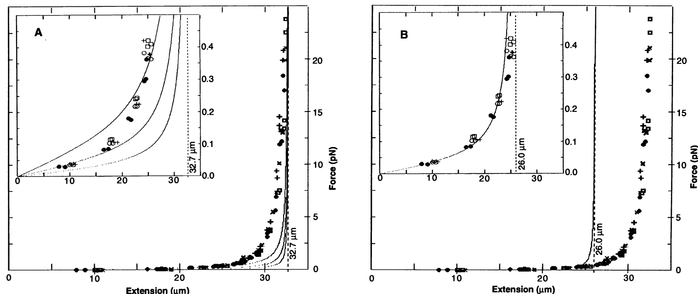
Fig. 3. (A) Force versus extension data for four different \lambda -dimer molecules (●, □, +, and ○) in 5 mM \text{Na}_2\text{HPO}_4 buffer (10 mM \text{Na}^+ , pH 8.3). Inset: expanded vertical scale (0 to 0.5 pN). Continuous curves are from Eq. 2 assuming L = 32.7 \mu\text{m} and b = 500 \text{ Å} (top), 1000 Å (middle), and
