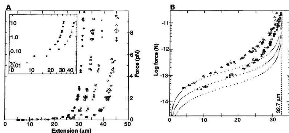
Fig. 5. (A) Force curves of a \lambda -dimer in 5 mM \text{Na}_2\text{HPO}_4 with various concentrations of ethidium bromide (Aldrich): ( \bullet ) unstained; ( \square ) 0.03 \mu\text{g/ml} ; ( \times ) 0.10 \mu\text{g/ml} ; ( \circ ) 1.0 \mu\text{g/ml} ; and ( + ) 2.0 \mu\text{g/ml} . If the intrinsic elastic properties of DNA do not change with intercalation, but molecules simply become longer by some factor, then the extensions would be increased by the same factor for all forces in the curve. In a log-log plot (see inset), the curve of the stained molecule would reproduce the curve of the native molecule but would be shifted to the right. Indeed, the curves are quite parallel except at the lowest forces where they diverge somewhat, perhaps because of an increasing persistence length with intercalation. The divergence, however, is close to the low-extension repeatability error of \pm 1 \text{ \mu m} . (B) Four native \lambda -dimers ( \bullet , \square , \times , and + ; same data as in Fig. 3), compared with three DDP-treated DNA molecules. Two of these are \lambda -monomers ( \Delta ), shown double length for comparison, and one is a \lambda -dimer ( \blacktriangle ). The DNA (concentration 400 ng/ml) and DDP (100 ng/ml) were reacted in 10 mM \text{NaClO}_4 buffer, in darkness, at 37^\circ\text{C} for 24 hours.
