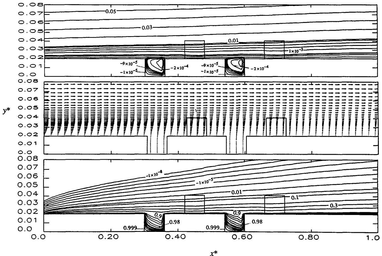
Figure 3 (a) Streamlines; (b) velocity distribution; and (c) isotherms for flow through alternate porous cavity-block obstacles for Re_L = 3 \times 10^4 , Da_L = 8 \times 10^{-6} , \Lambda_L = 0.35 , A = 3 , B = 1 , and H^* = 0.02
