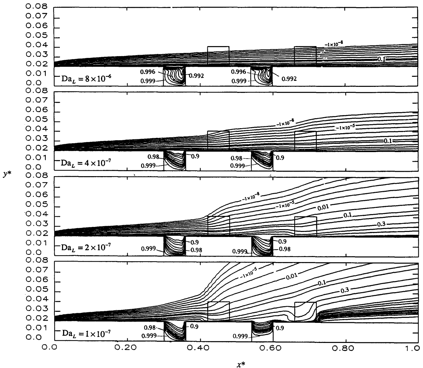
Figure 5 Effects of the Darcy number on isotherms for flow through alternate porous cavity-block obstacles for Re_L = 3 \times 10^5 , \Lambda_L = 0.35 , Pr = 0.7 , k_{eff}/k_f = 1.0 , A = 3 , B = 1 , H^* = 0.02
