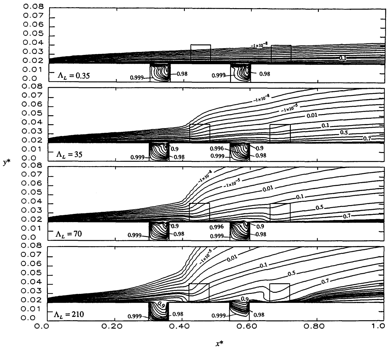
Figure 9 The influence of the inertial parameter on streamlines for flow through alternate porous cavity-block obstacles for Re_L = 3 \times 10^5 , Da_L = 8 \times 10^{-6} , A = 3 , B = 1 , H^* = 0.02
