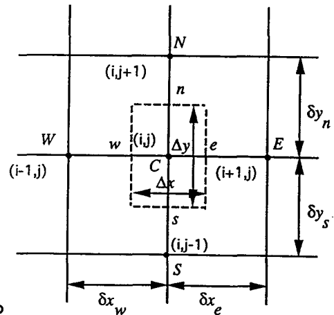
Figure 2 (a) Grid system for the computational domain; and (b) local integration cell
