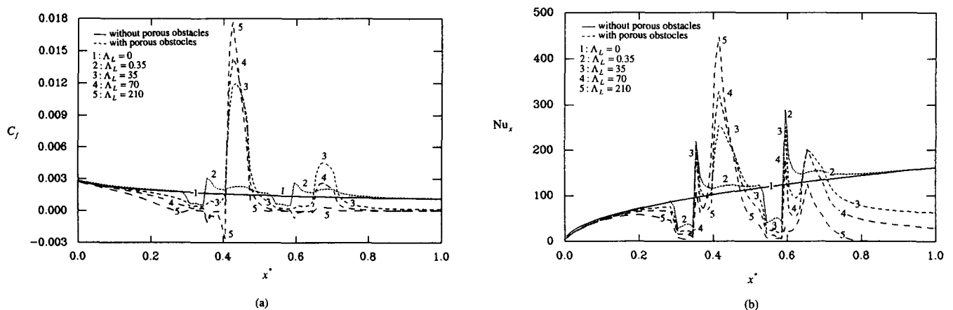
Figure 10 The influence of the inertial parameter on (a) friction coefficient and (b) Nusselt number for flow through alternate porous cavity-block obstacles for Re_L = 3 \times 10^5 , Da_L = 8 \times 10^{-6} , Pr = 0.7 , k_{eff}/k_f = 1.0 , A = 3 , B = 1 , H^* = 0.02
