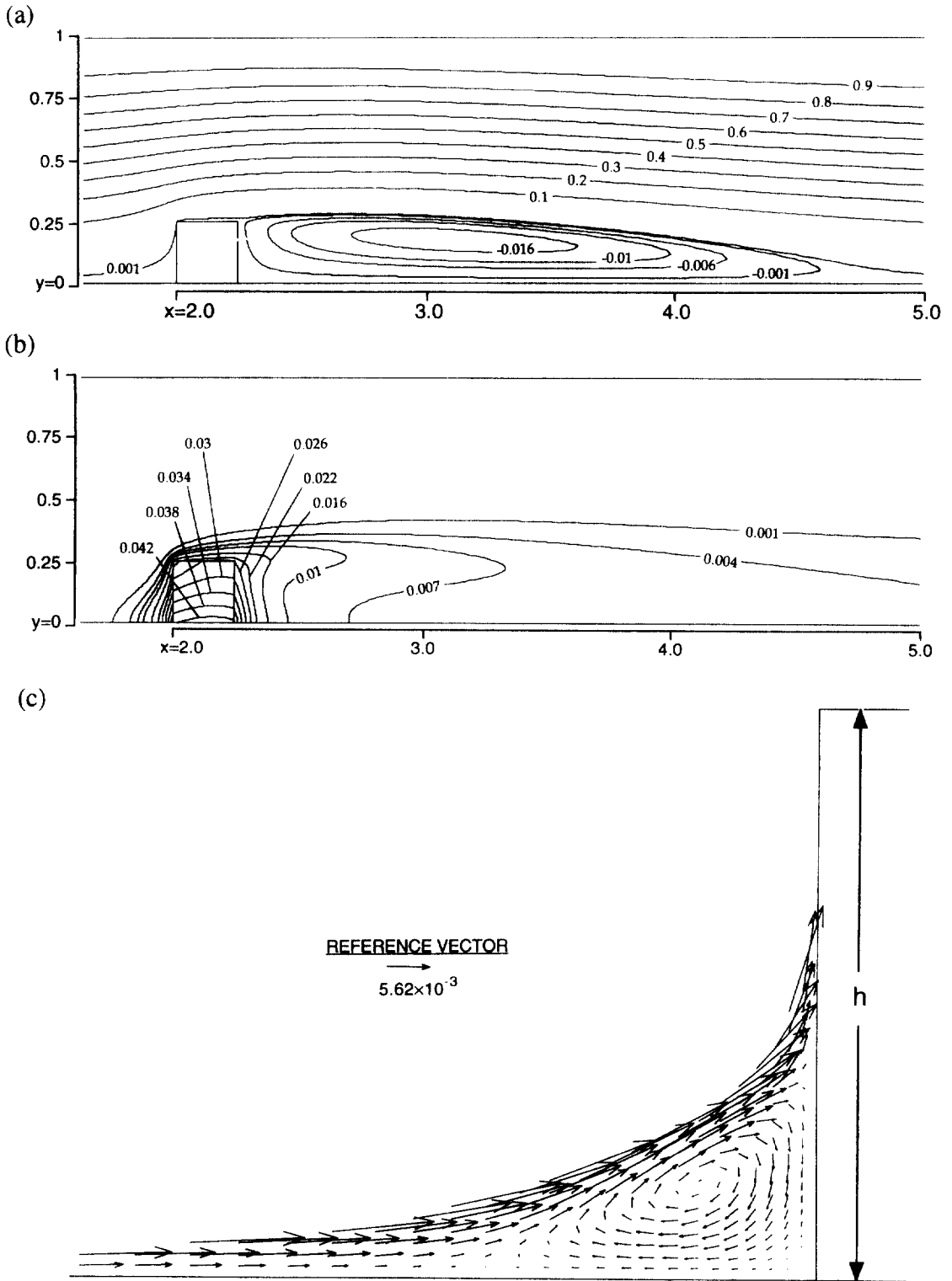
Fig. 3. Flow in a parallel plate channel with a solid, conducting obstacle for Re_{D_n} = 1000 , w = 0.25 , h = 0.25 , and k_s/k_f = 10 : (a) streamlines, (b) isotherms, and (c) close-up of upstream recirculation zone only showing vectors of the smallest magnitudes.
