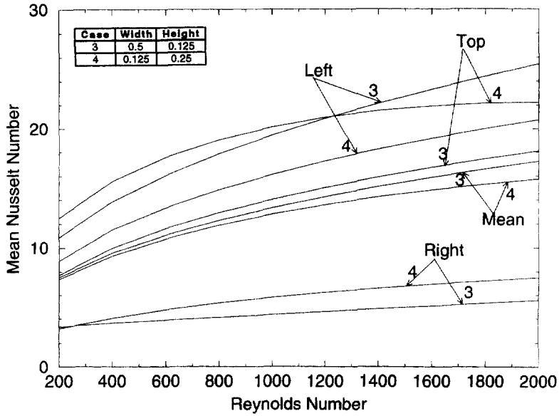
Fig. 13. Effects of obstacle shape variations on mean and exposed face mean Nusselt numbers versus Reynolds number for case 3 ( w = 0.5, h = 0.125 ) and case 4 ( w = 0.125, h = 0.25 ) with k_s/k_f = 1000 .
