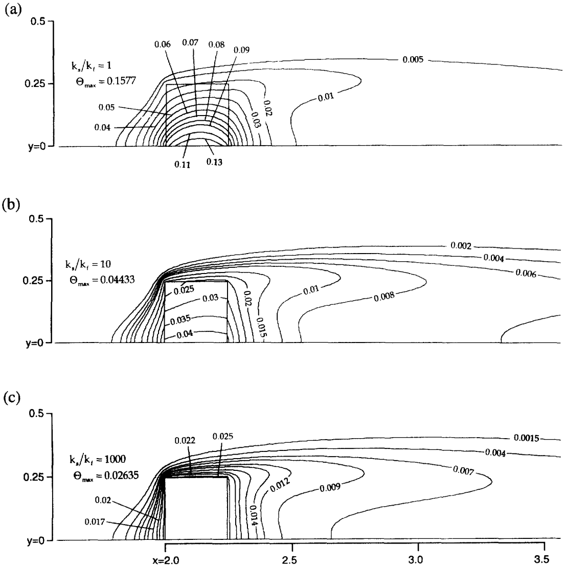
Fig. 8. Effects of the solid thermal conductivity on isotherms for flow in a parallel plate channel with a conducting obstacle for w = 0.25 , h = 0.25 , and Re_{D_h} = 1000 ; (a) k_s/k_f = 1 . (b) 10, and (c) 1000.
