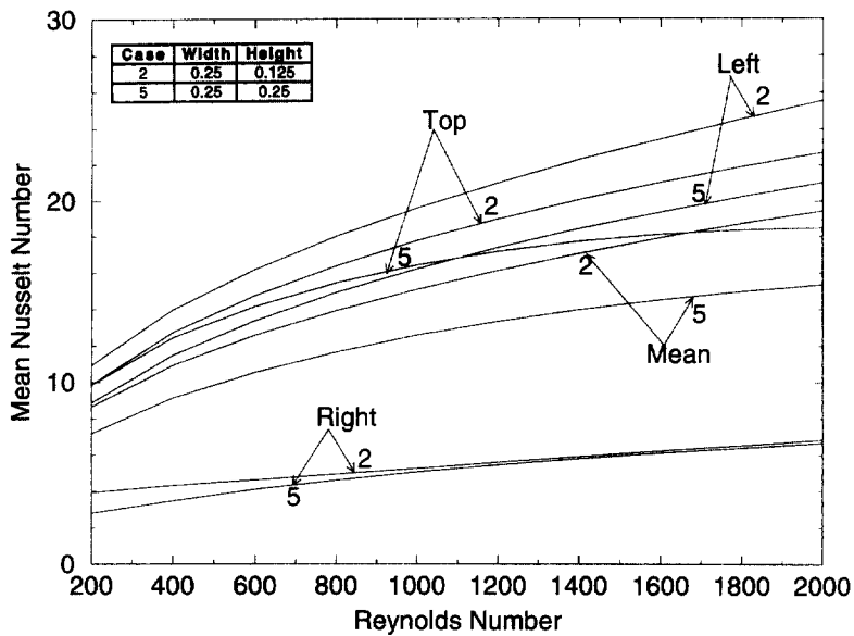
Fig. 12. Effects of obstacle height variations on mean and exposed face mean Nusselt numbers versus Reynolds number for case 2 ( w = 0.25, h = 0.125 ) and case 5 ( w = 0.25, h = 0.25 ) with k_s/k_f = 1000 .
