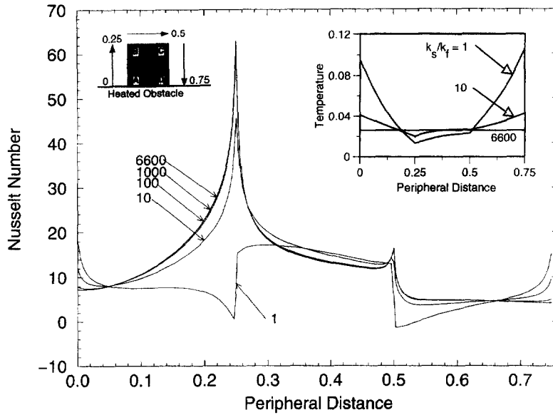
Fig. 9. Effects of variations in thermal conductivity ratio on local Nusselt number distributions around the obstacle periphery for w = 0.25, h = 0.25, Re_{D_s} = 1000, and 1 \leq k_s/k_t \leq 6600 . The inset shows the obstacle surface temperatures for various k_s/k_t .
