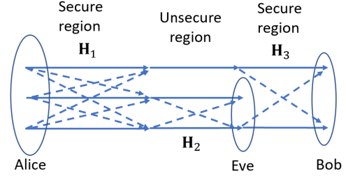
Fig. 2. Wireline channels where GCP and GPP could be applied if \text{range}(\mathbf{H}_{B,A}^T) \not\subset \text{range}(\mathbf{G}_A^T) with \mathbf{H}_{B,A} = \mathbf{H}_3 \text{diag}(1, \mathbf{H}_2) \mathbf{H}_1 and \mathbf{G}_A = \mathbf{H}_2 \mathbf{H}_1 . Here three strongly coupled wires originated from Alice traverse separately over a wide unsecured field while two of them are wiretapped by Eve and two of them are eventually connected to Bob. A randomized \mathbf{H}_1 could be artificially generated by Alice even if \mathbf{H}_2 and \mathbf{H}_3 become selection matrices due to good insulation between wires.
