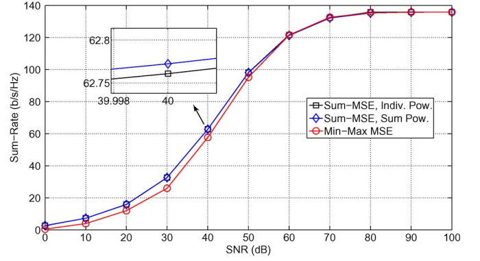
Fig. 4. Sum-rate comparison of the proposed algorithm versus SNR. Here, N=2 , K=3 , \kappa=\beta=-40 dB, \text{INR}=10 dB, \text{INR}_{\text{SI}}=20 dB, \mu=0 dB, \lambda=0 dB.
