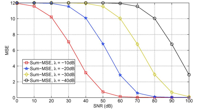
Fig. 7. MSE of cognitive radio system with different \lambda values versus SNR. Here, N = 2 , K = 3 , \kappa = \beta = -40 dB, \text{INR} = 10 dB, \text{INR}_{\text{SI}} = 20 dB, \mu = 0 dB.
