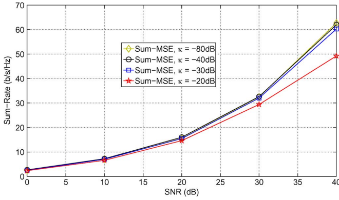
Fig. 6. Sum-rate comparison of the Sum-MSE algorithm with different \kappa = \beta values versus SNR. Here, N = 2 , K = 3 , \text{INR} = 10 dB, \text{INR}_{\text{SI}} = 20 dB, \mu = 0 dB, \lambda = 0 dB.
