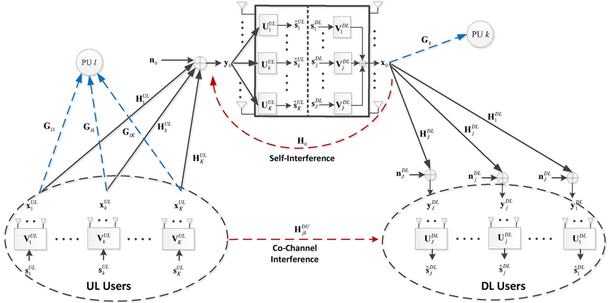
Fig. 2. Full-duplex multi-user MIMO system model.
