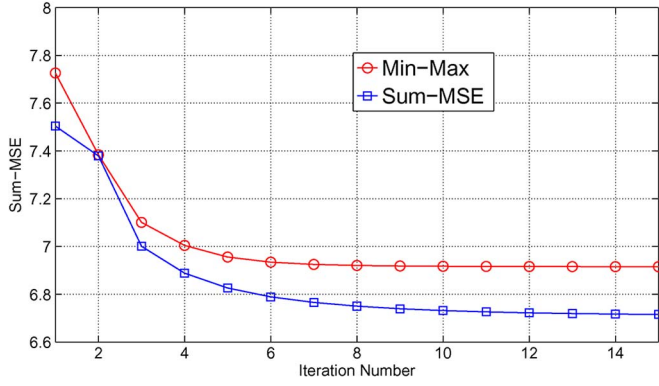
Fig. 3. Convergence behavior of Sum-MSE and Min-Max algorithms. Here, N=2 , K=3 , \kappa=\beta=-40 dB, \text{SNR}=20 dB, \text{INR}=10 dB, \text{INR}_{\text{SI}}=20 dB, \mu=0 dB, \lambda=0 dB.
