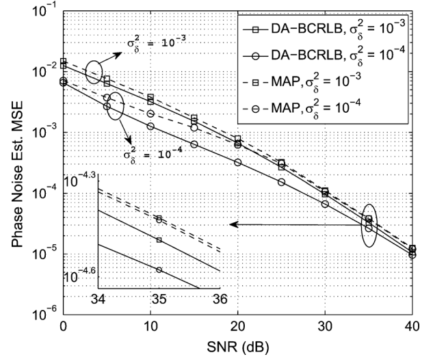
Fig. 5. Online MAP estimator's MSE and DA-BCRLB versus SNR for a 2 \times 2 MIMO system with \sigma_\delta^2 = [10^{-3}, 10^{-4}] \text{ rad}^2 and K = 20 .
