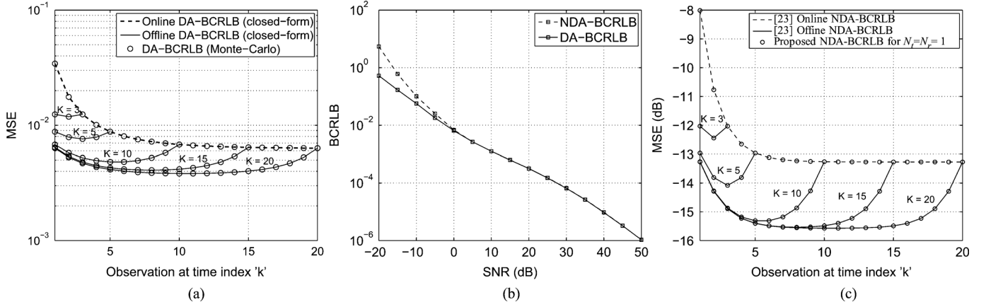
Fig. 2. (a) Online and offline DA-BCRLB versus the number of observations for 2 \times 2 MIMO system with \text{SNR} = 5 dB and \sigma_\delta^2 = 10^{-3} \text{ rad}^2 . (b) NDA- and DA-BCRLB for 2 \times 2 MIMO system versus SNR evaluated at k = 20 in a frame of K = 20 symbols with \sigma_\delta^2 = 10^{-4} \text{ rad}^2 . (c) Comparison of derived online and offline NDA-BCRLB results with [23] for \text{SNR} = 5 dB, N_t = N_r = 1 , and \sigma_\delta^2 = 10^{-2} \text{ rad}^2 .
