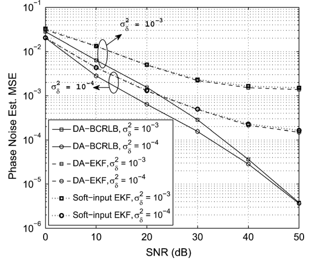
Fig. 6. EKF's MSEs and the DA-BCRLB versus SNR for a 2 \times 2 MIMO system with \sigma_\delta^2 = [10^{-3}, 10^{-4}] \text{ rad}^2 and K = 20 .
