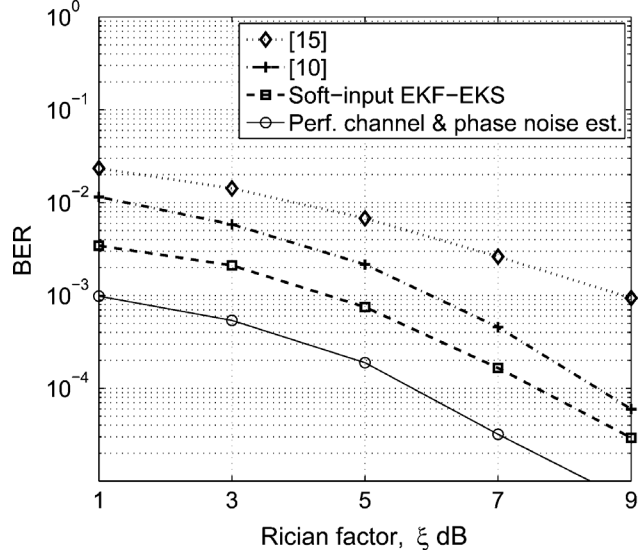
Fig. 10. BER of a 2 \times 2 MIMO system as a function of the Rician factor, \xi , for BPSK modulation, \sigma_\delta^2 = 10^{-4} \text{ rad}^2 , and SNR = 10 dB.
