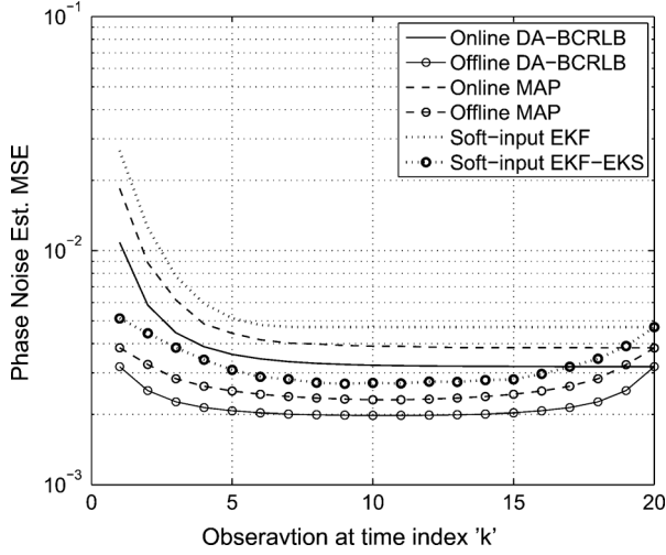
Fig. 4. Phase noise estimation MSEs and BCRLB versus observation index, k , for a 2 \times 2 MIMO system with \sigma_\delta^2 = 10^{-3} \text{ rad}^2 , SNR = 10 dB, and K = 20 .
