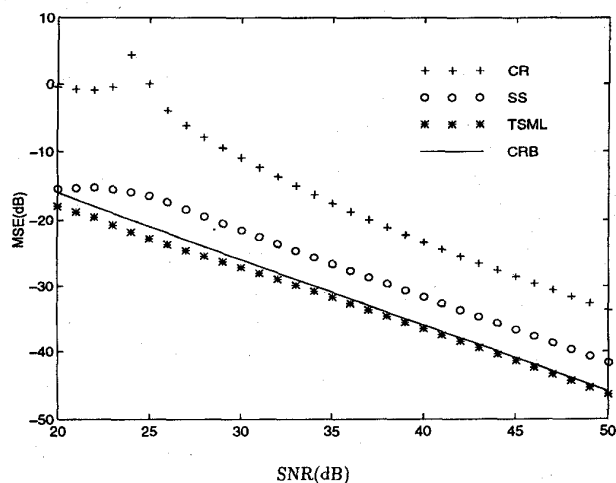
Fig. 5. Performances of the CR, SS, and TSML methods versus SNR, where \delta = \pi/10 and \theta = \pi/10 , and the first step of the TSML method was replaced by the SS method.
