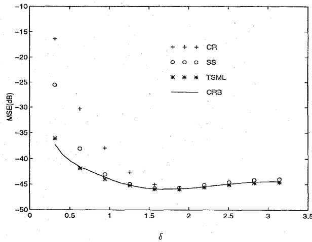
Fig. 1. Performances of the CR, SS, and TSML methods versus \delta , where SNR = 45 dB, and \theta = 0 .
