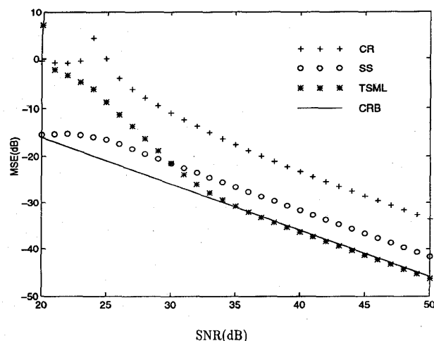
Fig. 4. Performances of the CR, SS, and TSML methods versus SNR, where \delta = \pi/10 , and \theta = \pi/10 .
