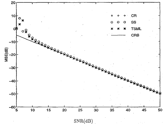
Fig. 3. Performances of the CR, SS, and TSML methods versus SNR, where \delta = \pi , and \theta = \pi/10 .
