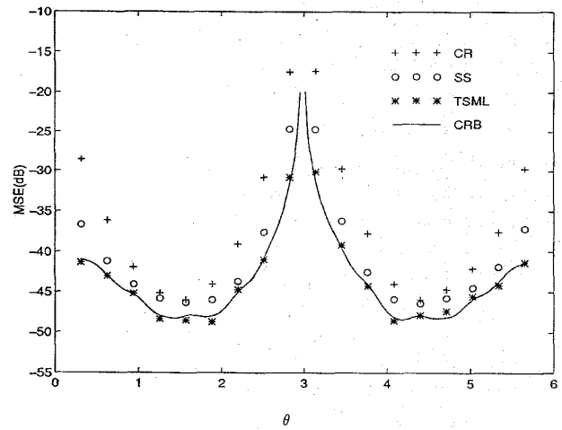
Fig. 2. Performances of the CR, SS, and TSML methods versus \theta , where SNR = 45 dB, and \delta = \pi/11 .
